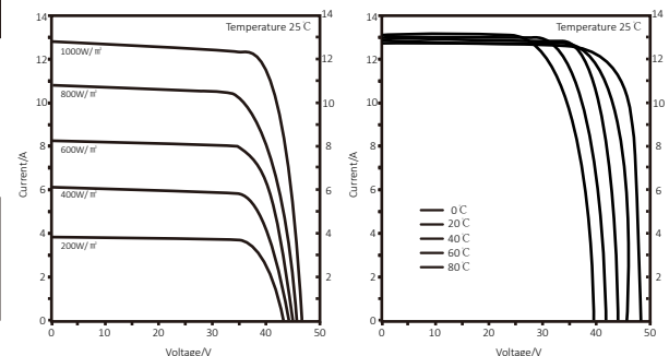
Current-Voltage Curve (BSM500PM5-72SB)
